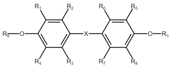
(B) Bisphenol derivative structure
